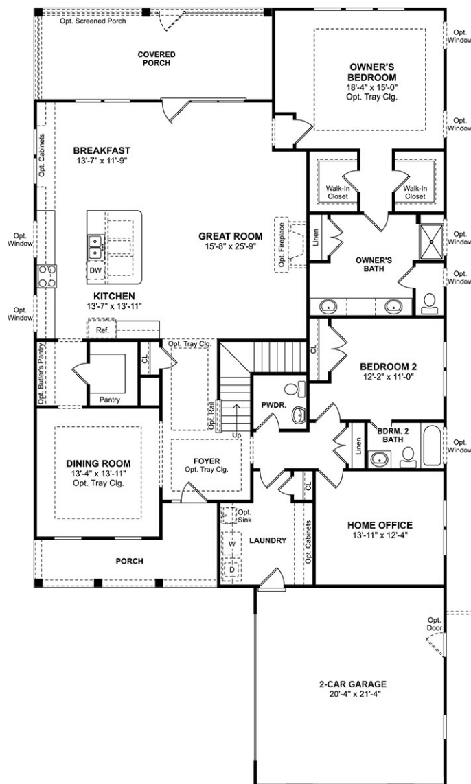
MAIN LEVEL
