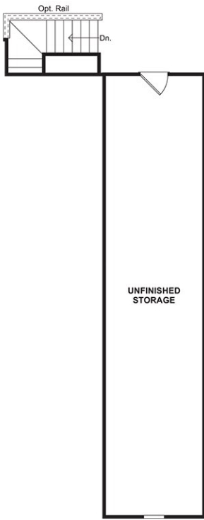
OPTIONAL EXTENDED ATTIC STORAGE
