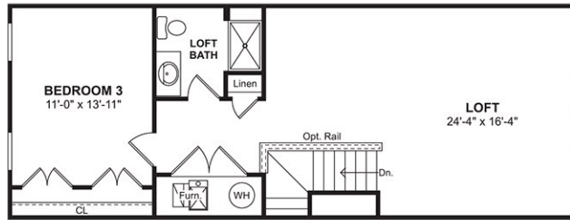
UPPER LEVEL
